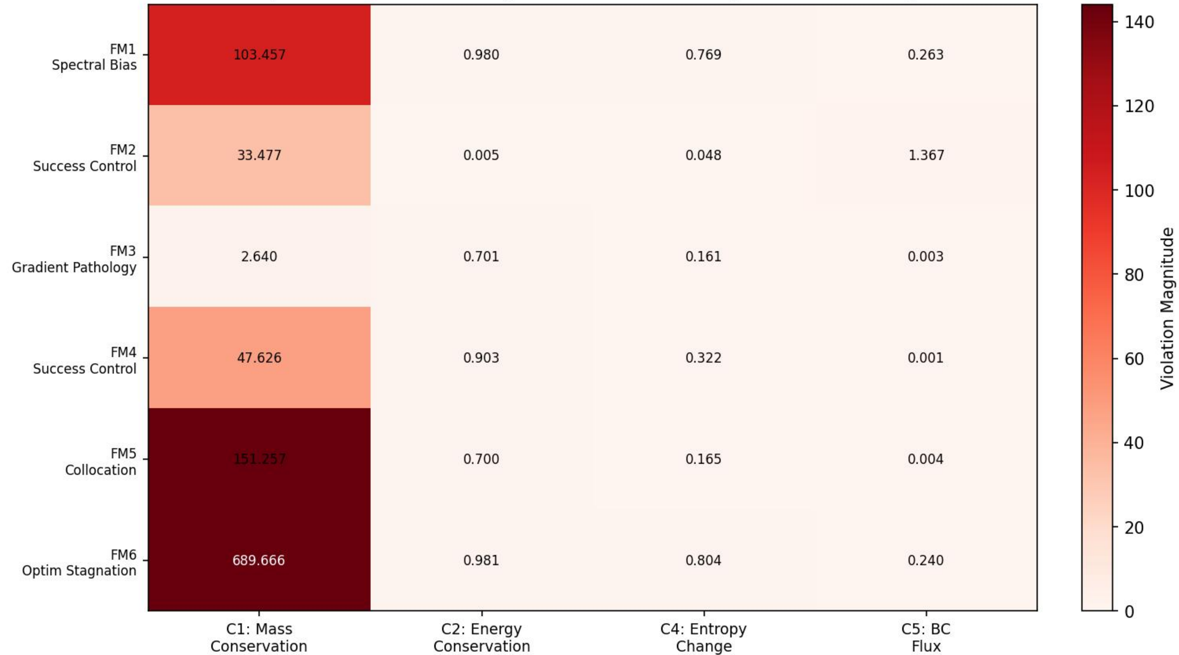
Conservation Law Violation Heatmap (Final-time violations, row = failure mode, col = invariant)
