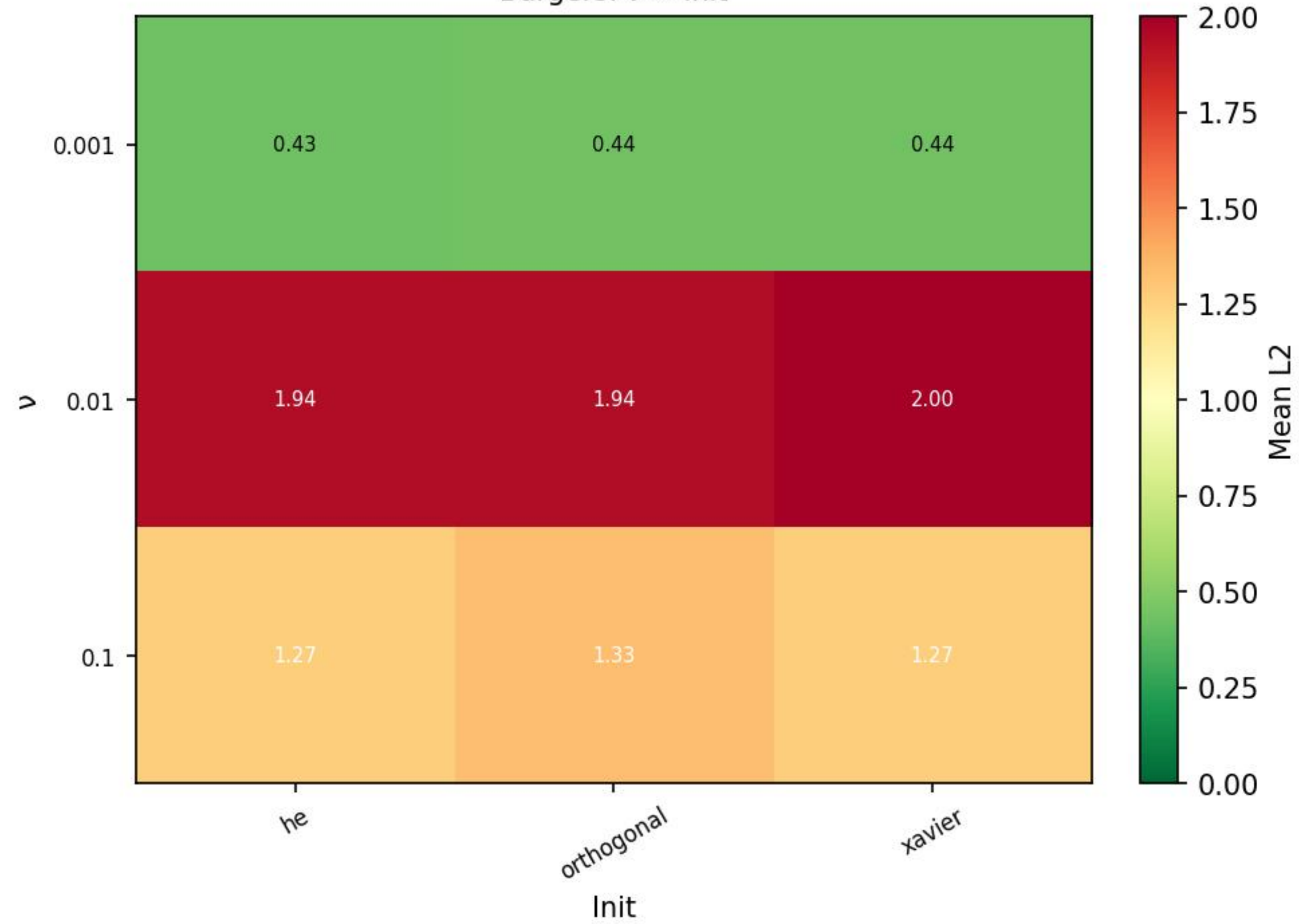
Burgers: \nu \times \text{Init}
