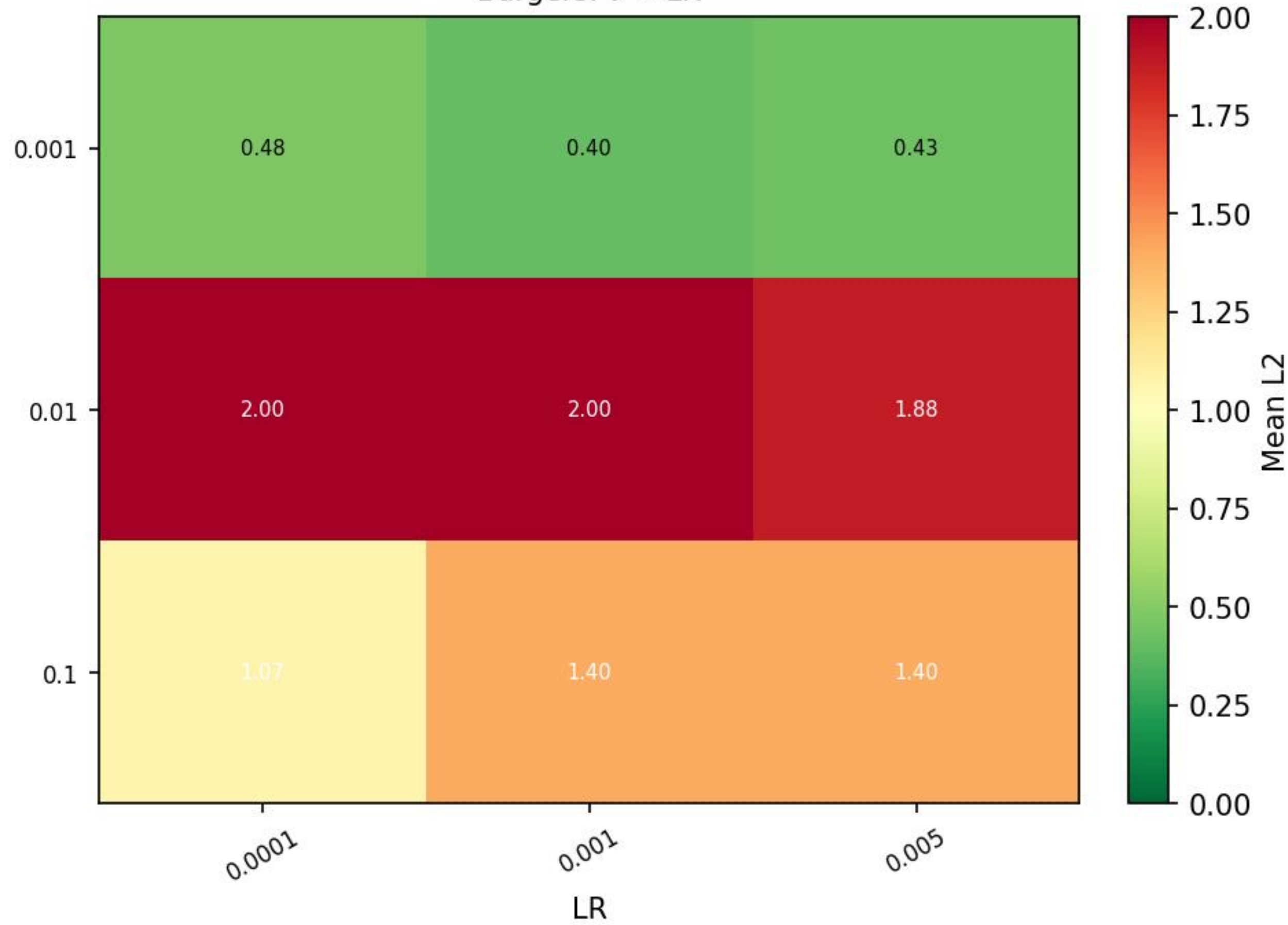
Burgers: \nu \times \text{LR}
