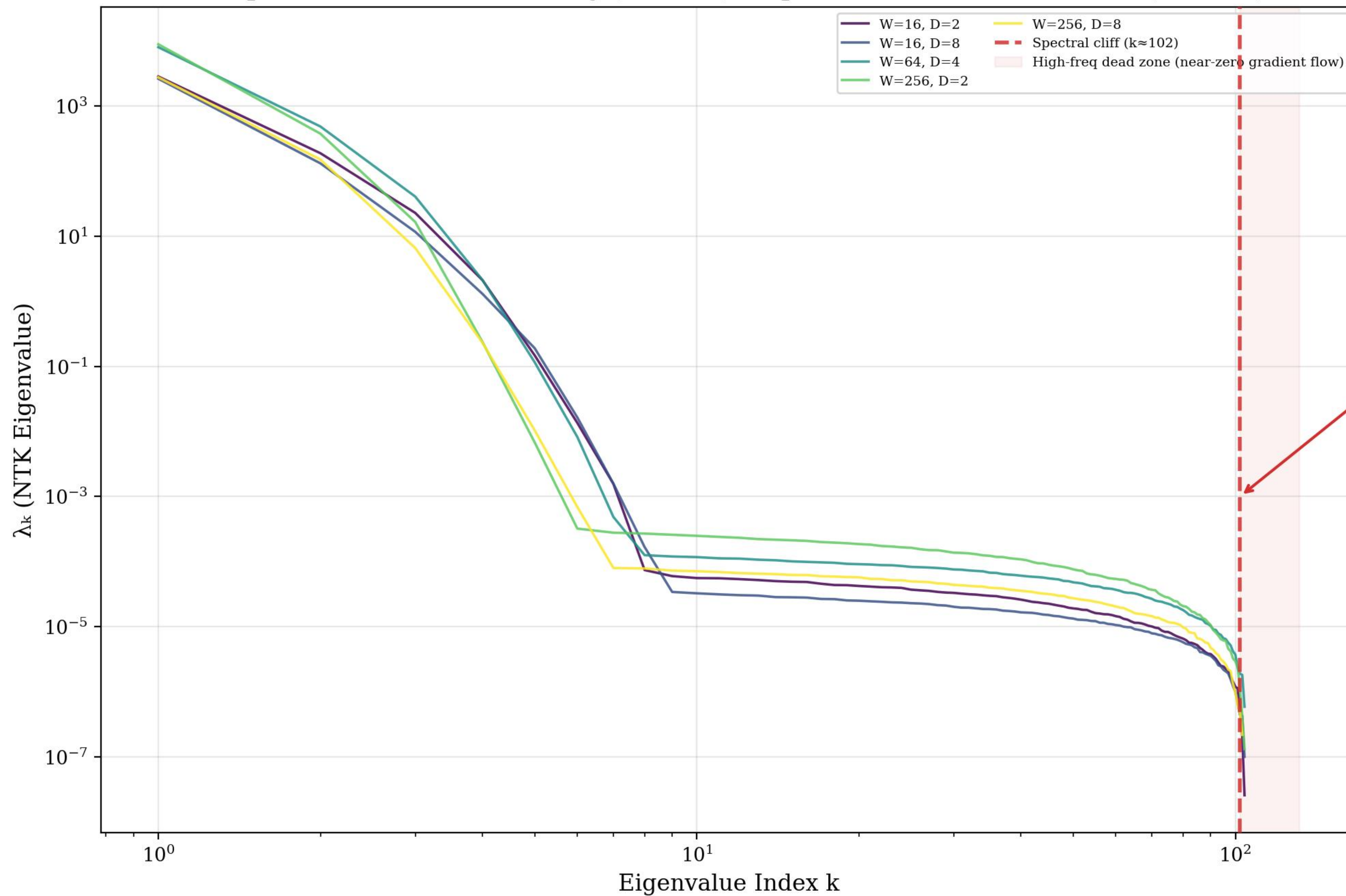
NTK Eigenvalue Spectra by Architecture — at initialization Two-phase structure: bulk decay ( k < \text{cliff} ) \rightarrow spectral cliff \rightarrow near-zero tail ( k > \text{cliff} )
