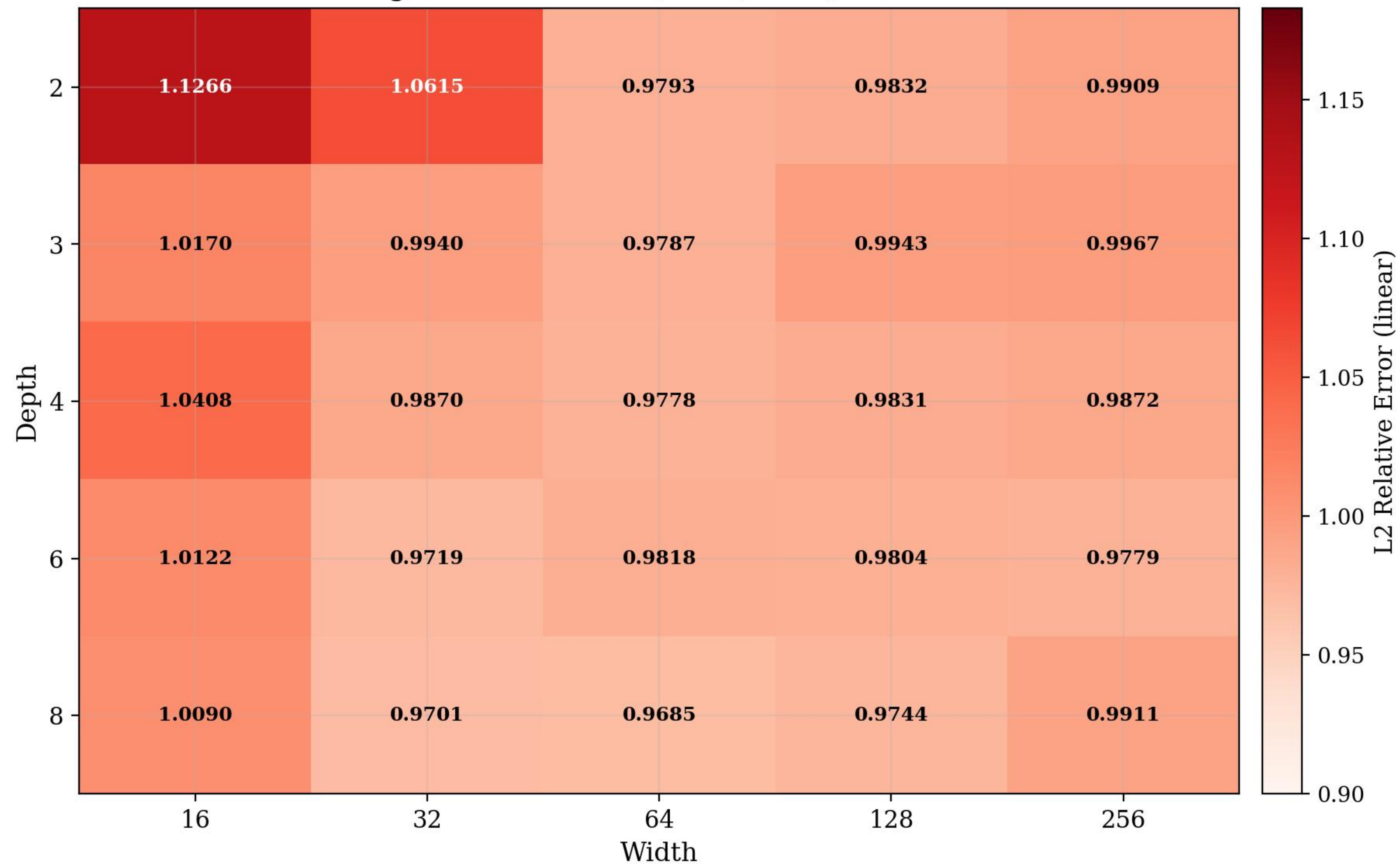
L2 Relative Error ( \beta=50 ) [linear scale] All 25 configurations fail: L2 \in [0.969, 1.127] \gg 0.1 threshold
