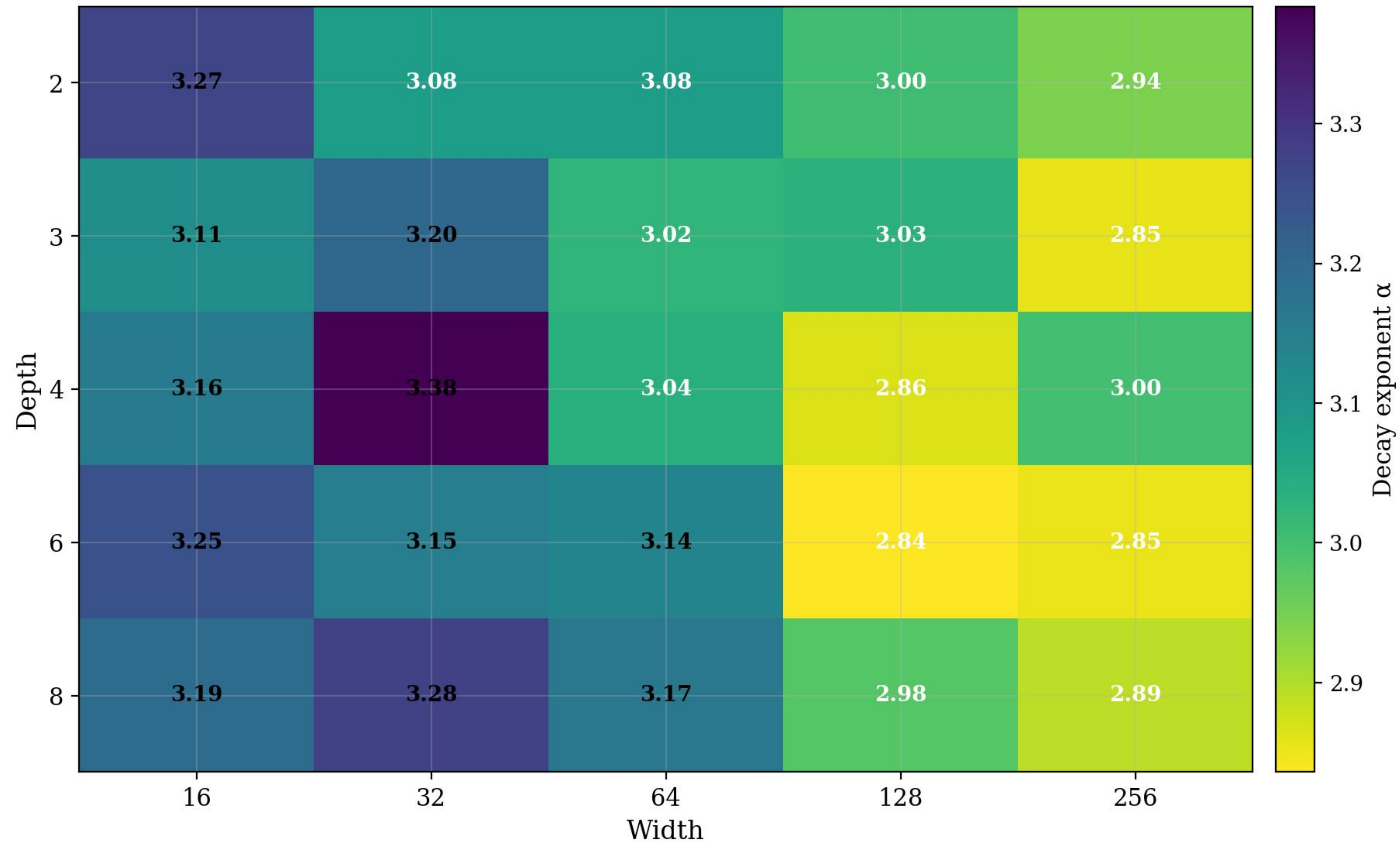
NTK Spectral Decay Exponent \alpha — at initialization ( \lambda_k \sim k^{-\alpha} ; higher \alpha = steeper decay = stronger spectral bias) Width=256 slightly reduces \alpha (2.89 vs 3.35) — insufficient to cure failure
