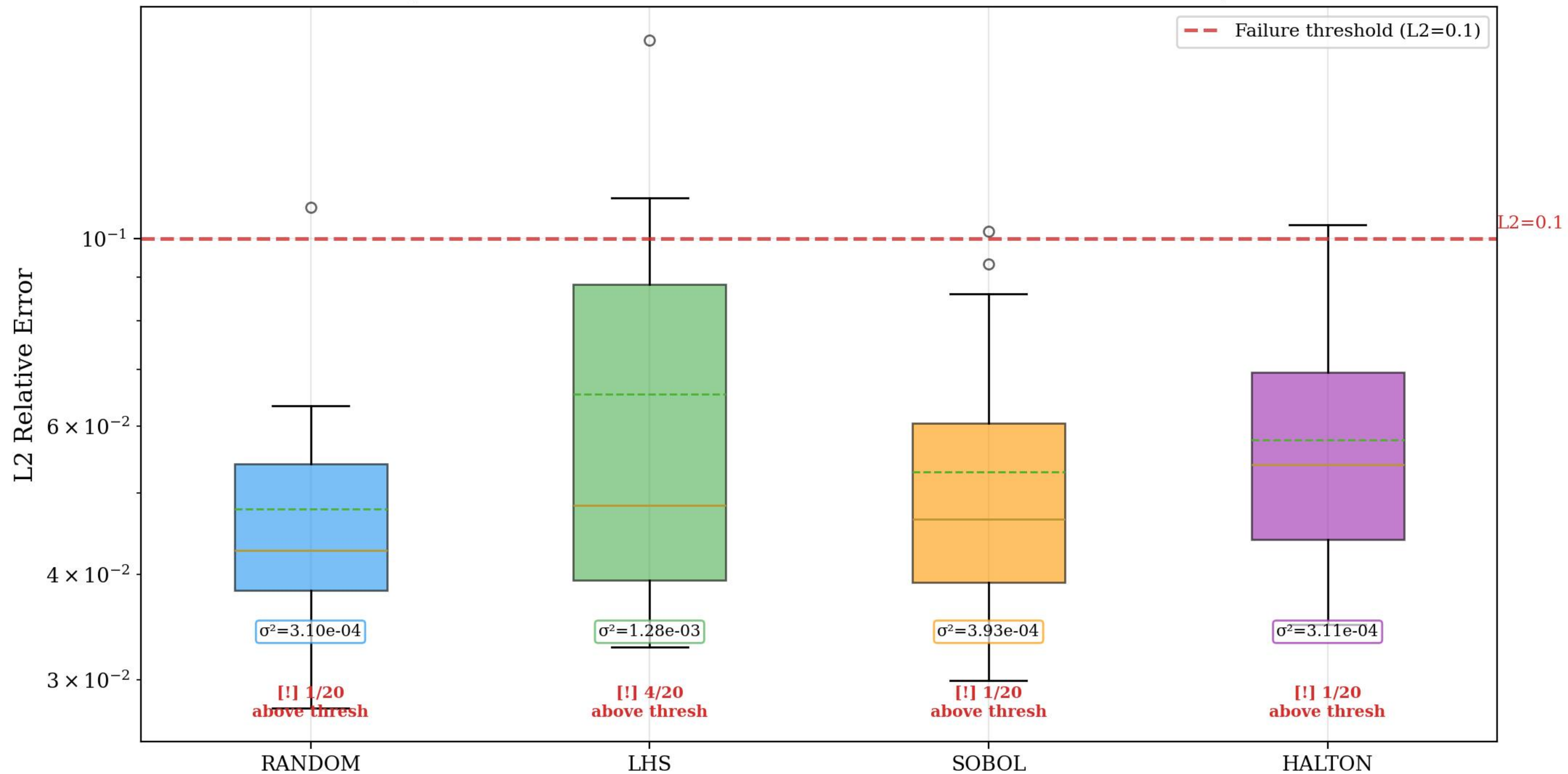
Final L2 Error Distribution by Sampling Strategy (20 seeds each. [!] = seeds above L2=0.10 failure threshold.)
