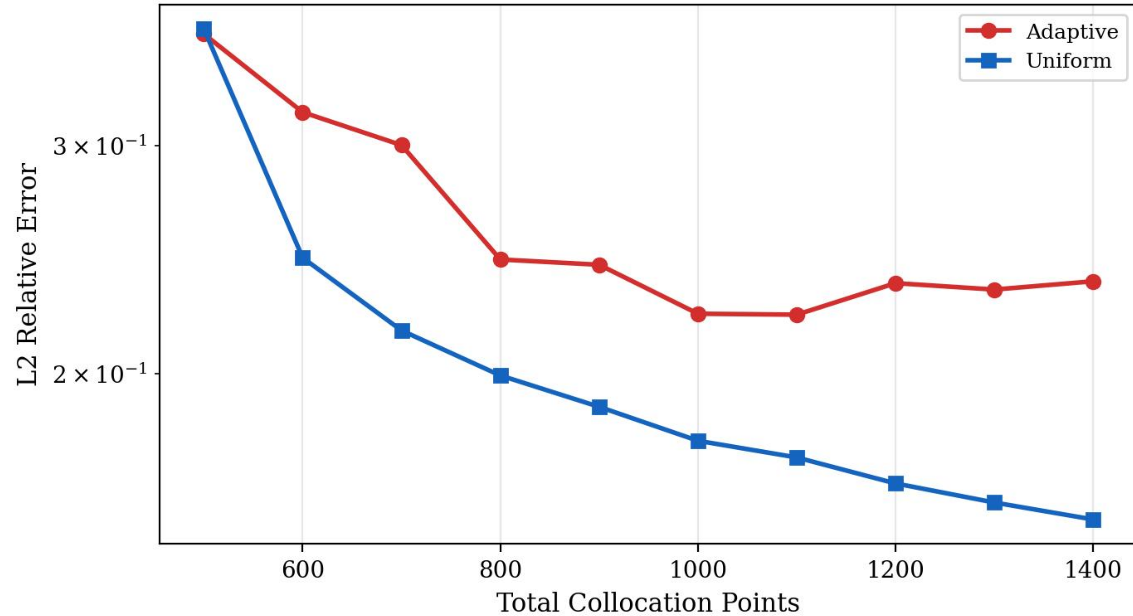
L2 Error vs Total Point Budget
