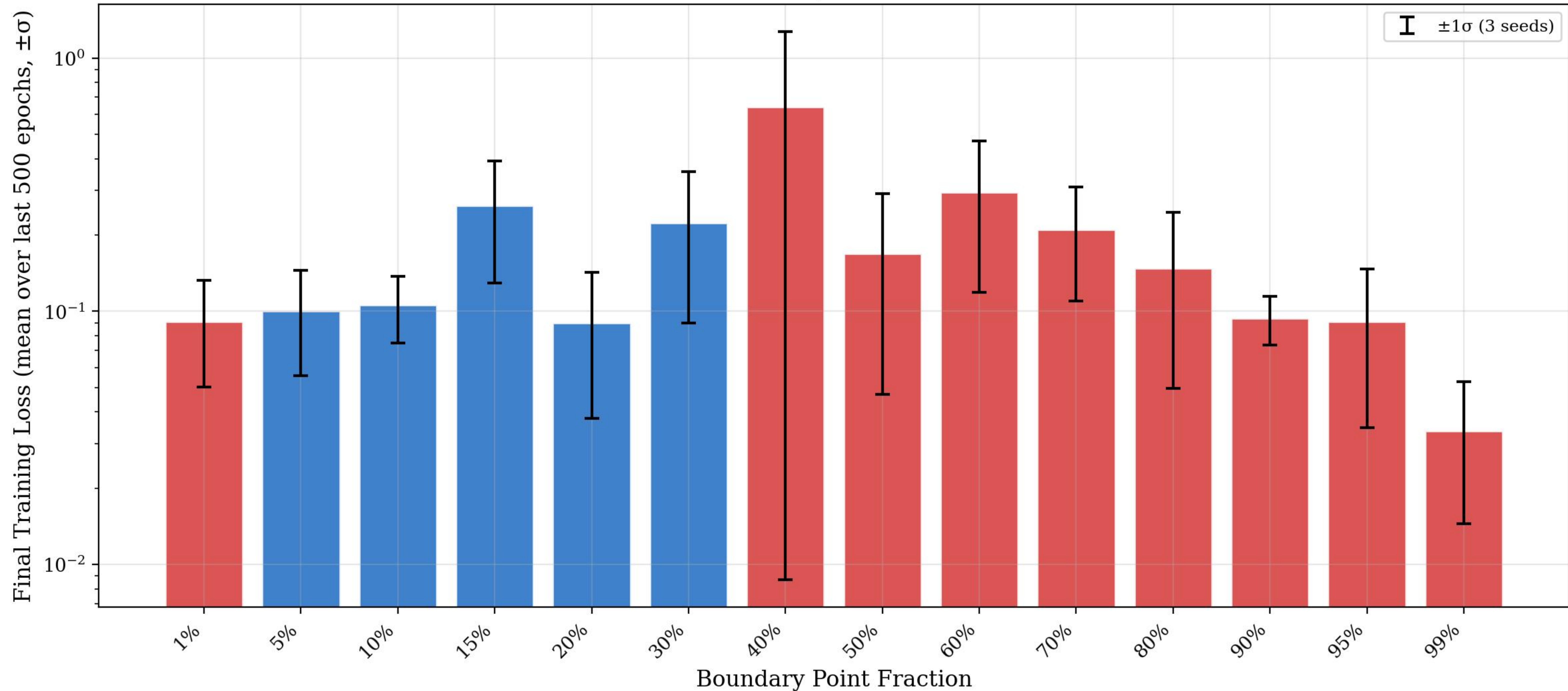
Final Training Loss vs Boundary/Interior Ratio (Replaces 'convergence epoch' which was uniformly 10000 in v1 — the loss threshold was never crossed) Red=FAIL, Blue=PASS.
