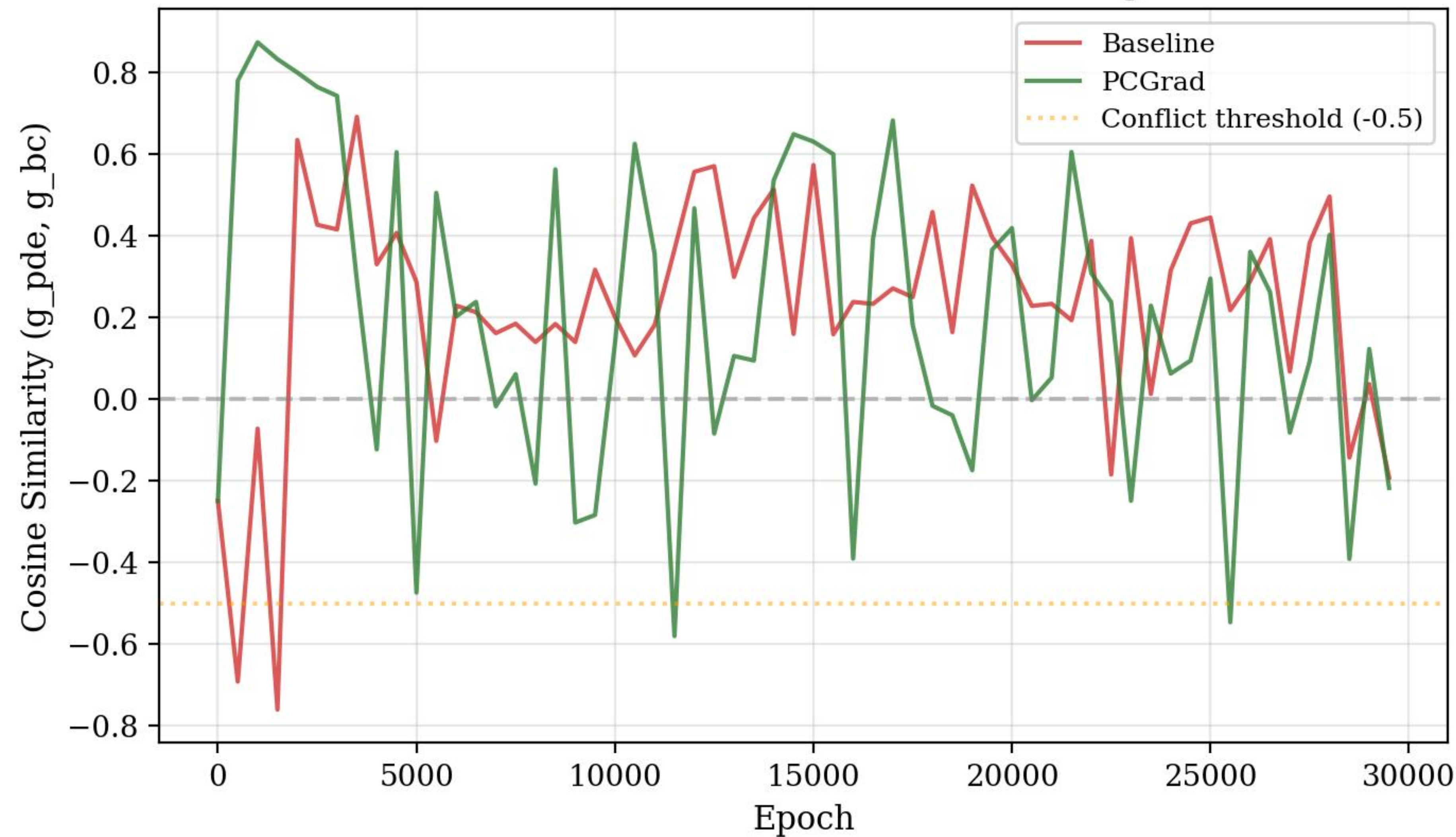
Gradient Conflict Over Training
