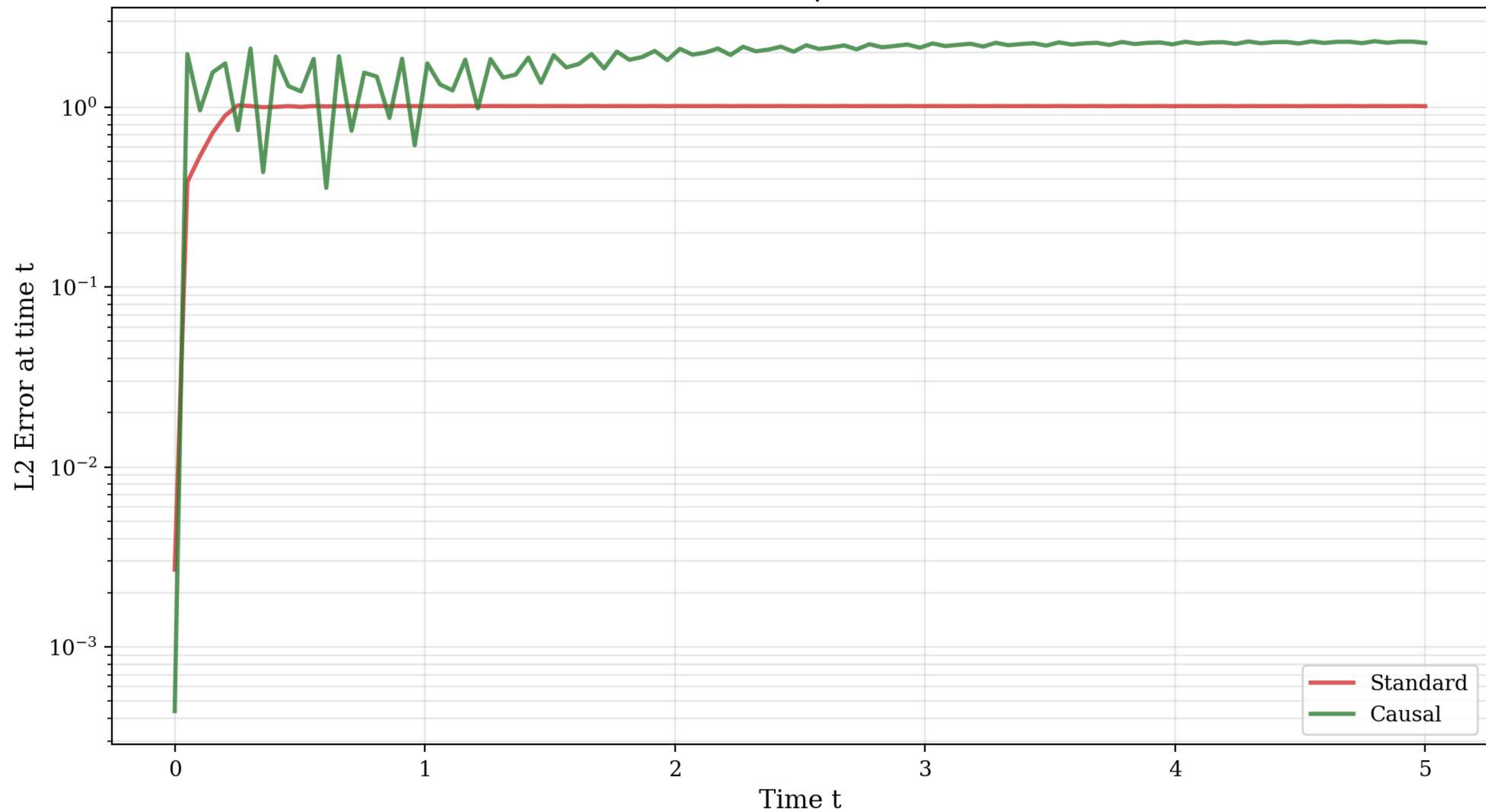
Causal Training vs Standard ( \beta=50 , t \in [0,5] ) Standard L2=0.9955 | Causal L2=1.9815
