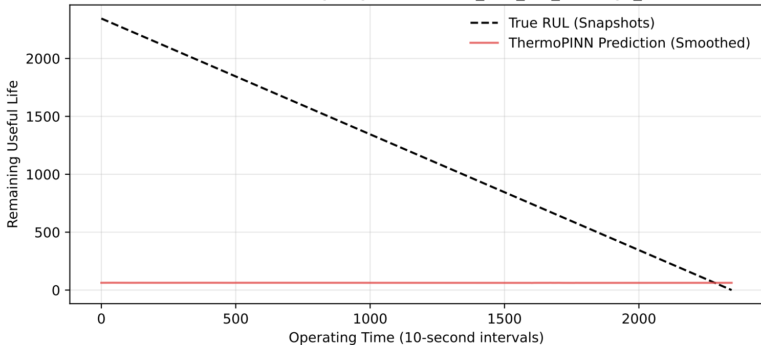
Zero-Shot Bearing Degradation: Full_Test_Set_Bearing1_3
