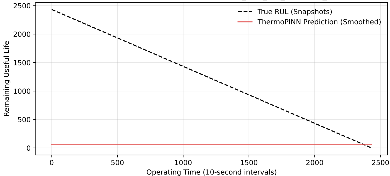
Zero-Shot Bearing Degradation: Full_Test_Set_Bearing1_5
