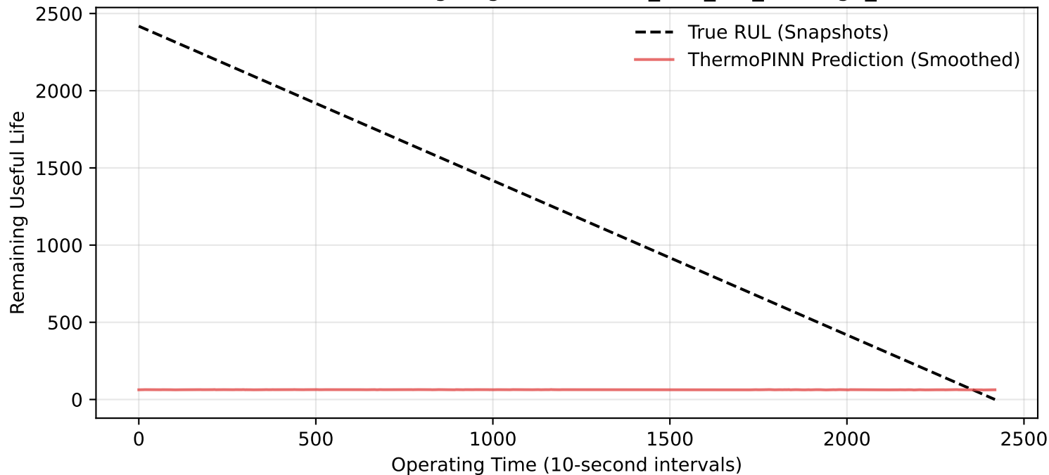
Zero-Shot Bearing Degradation: Full_Test_Set_Bearing1_6
