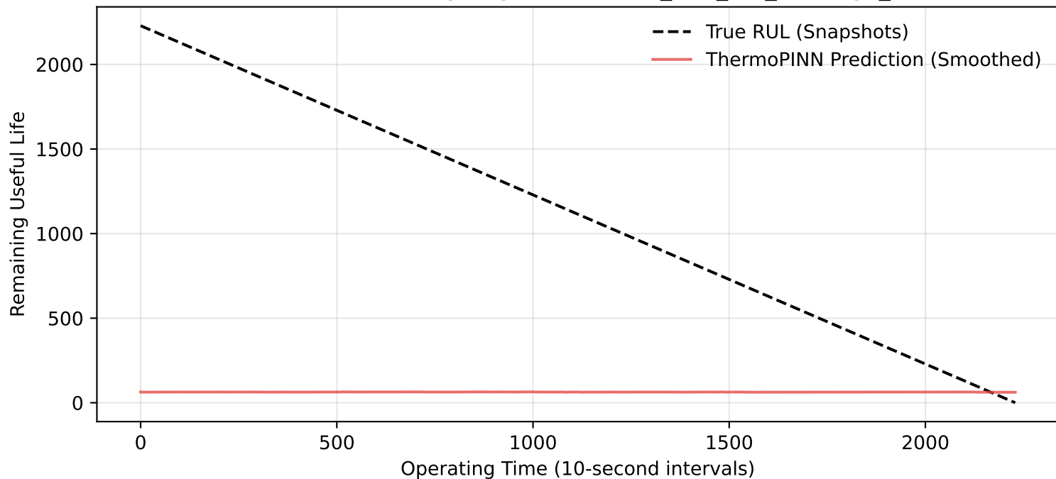
Zero-Shot Bearing Degradation: Full_Test_Set_Bearing1_7
