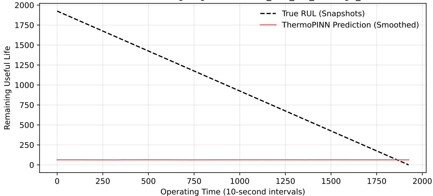
Zero-Shot Bearing Degradation: Full_Test_Set_Bearing2_3
