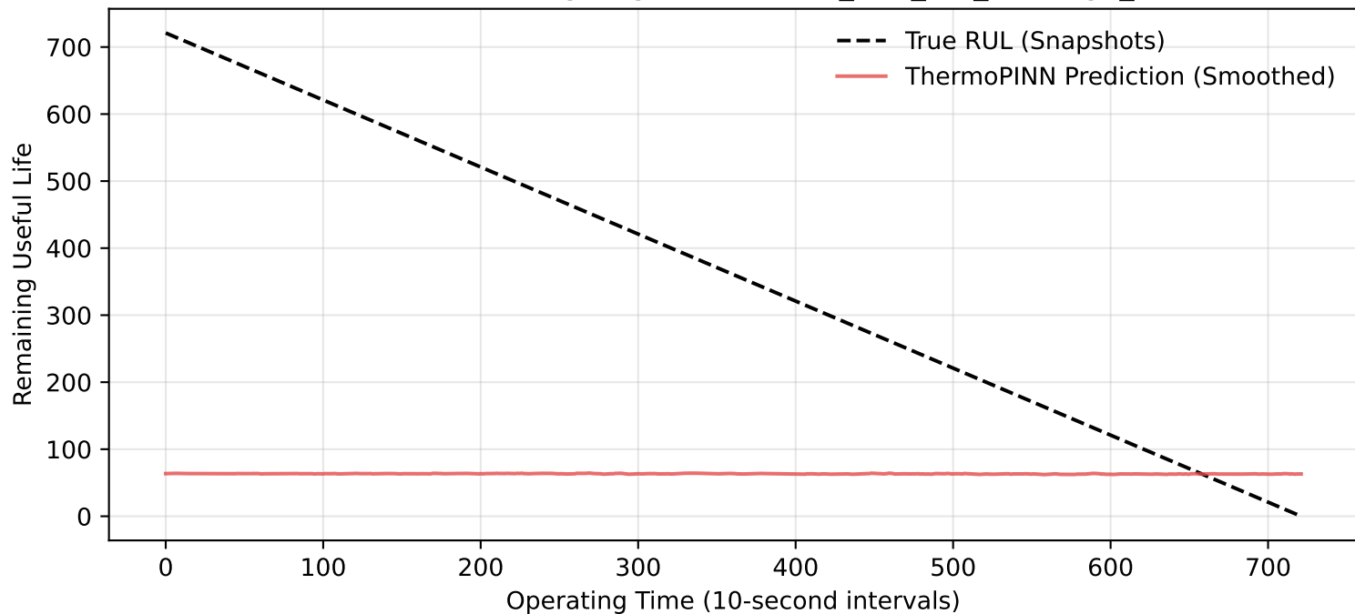
Zero-Shot Bearing Degradation: Full_Test_Set_Bearing2_4
