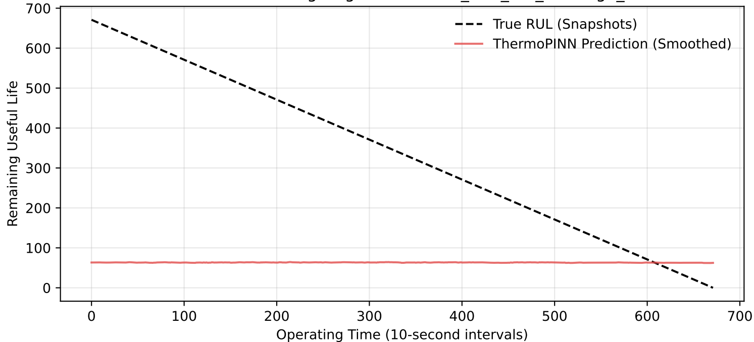
Zero-Shot Bearing Degradation: Full_Test_Set_Bearing2_6
