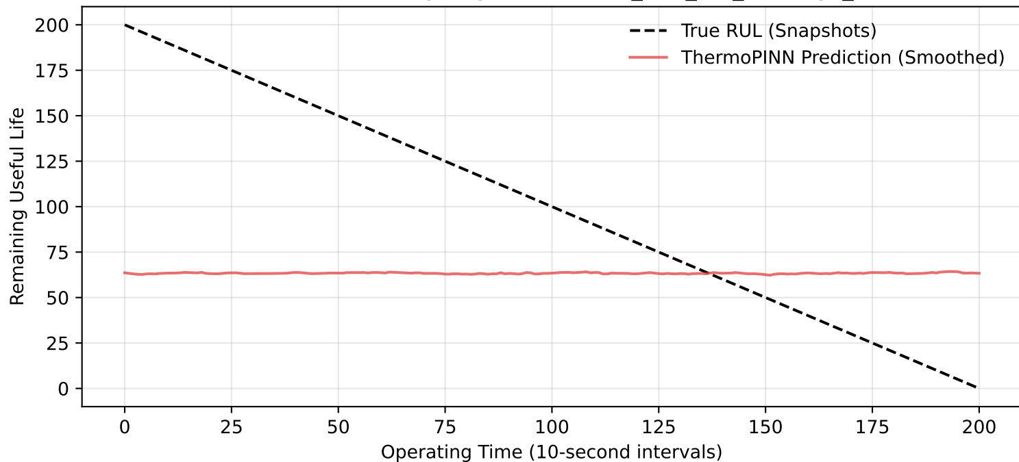
Zero-Shot Bearing Degradation: Full_Test_Set_Bearing2_7
