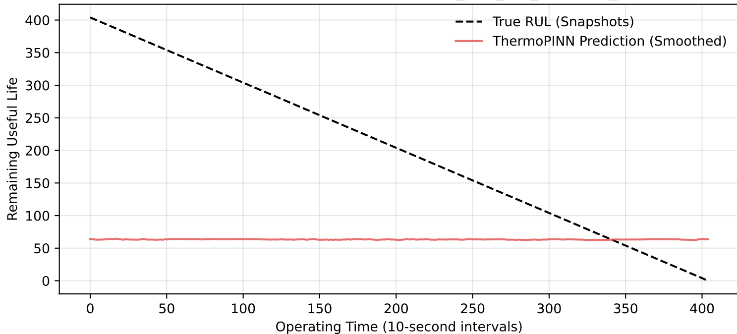
Zero-Shot Bearing Degradation: Full_Test_Set_Bearing3_3
