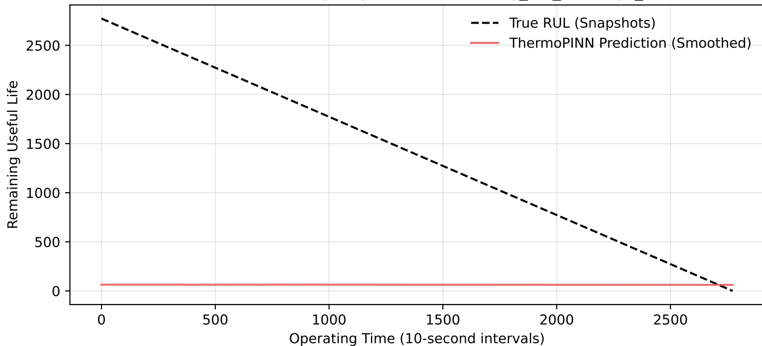
Zero-Shot Bearing Degradation: Learning_set_Bearing1_1
