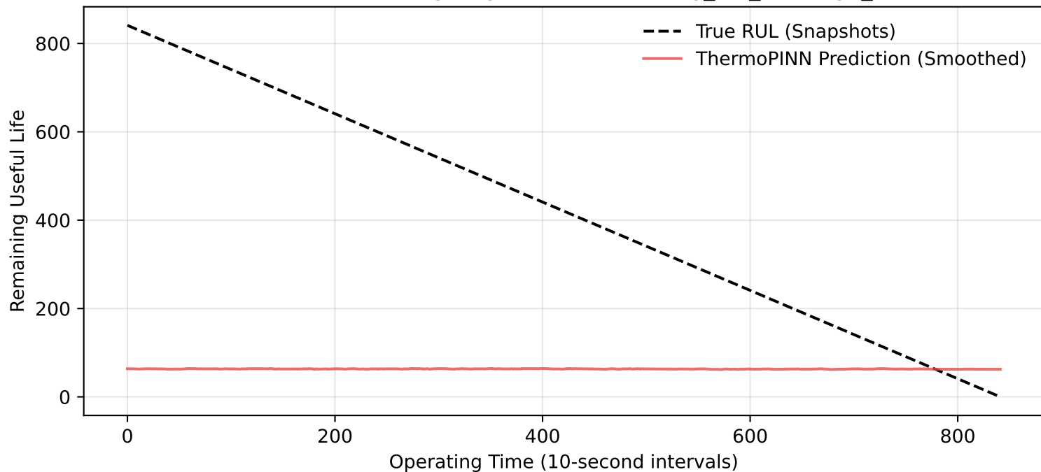
Zero-Shot Bearing Degradation: Learning_set_Bearing1_2
