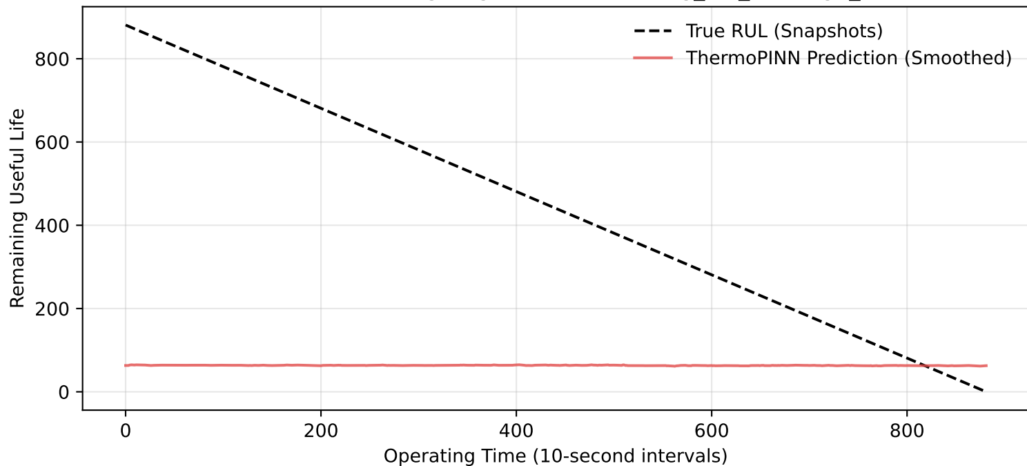
Zero-Shot Bearing Degradation: Learning_set_Bearing2_1
