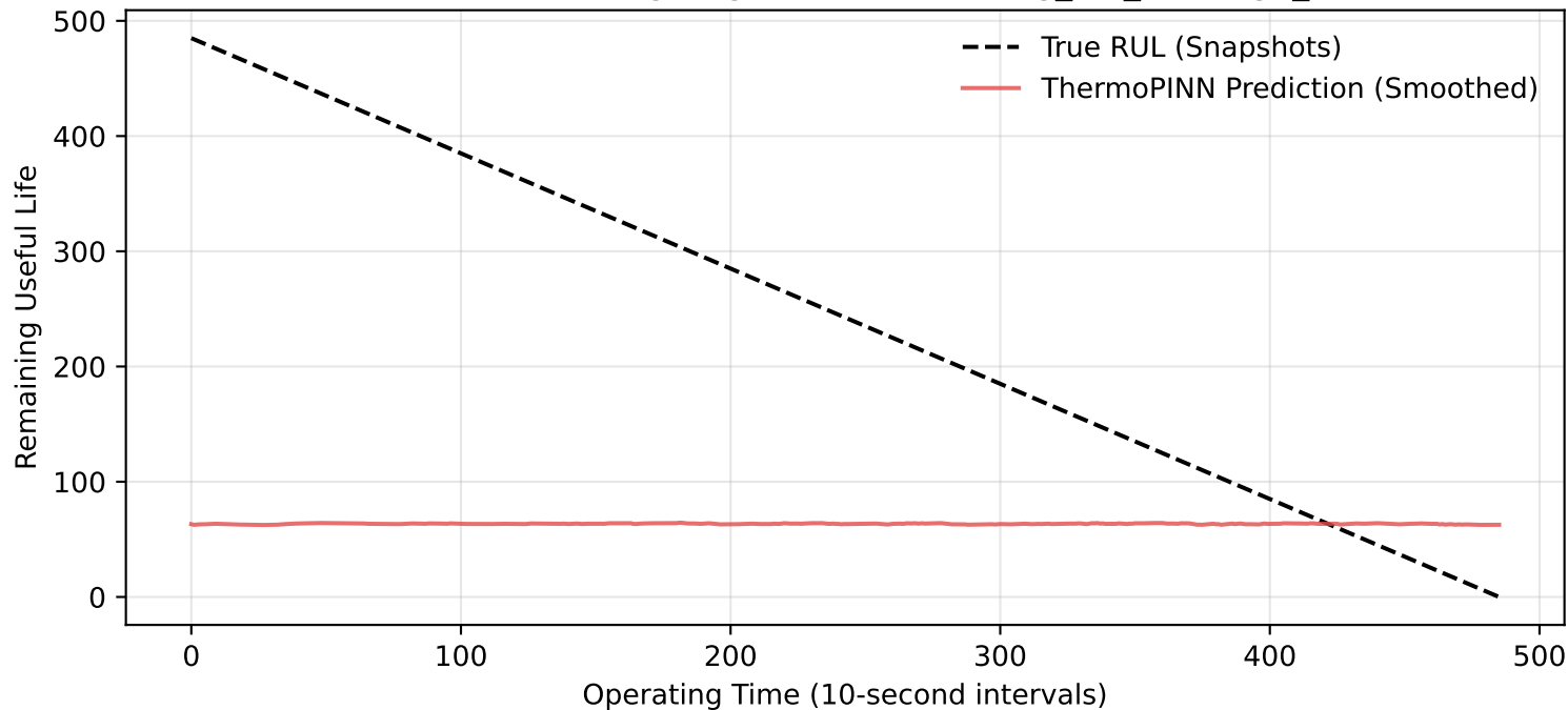
Zero-Shot Bearing Degradation: Learning_set_Bearing3_1
