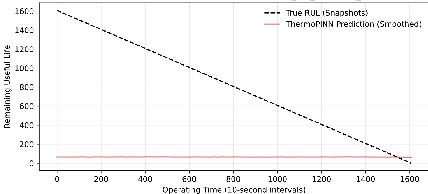
Zero-Shot Bearing Degradation: Learning_set_Bearing3_2
