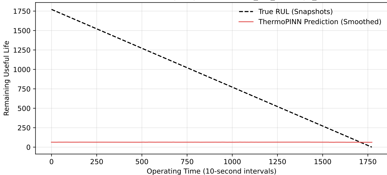
Zero-Shot Bearing Degradation: Test_set_Bearing1_3
