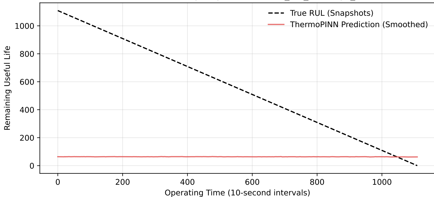
Zero-Shot Bearing Degradation: Test_set_Bearing1_4
