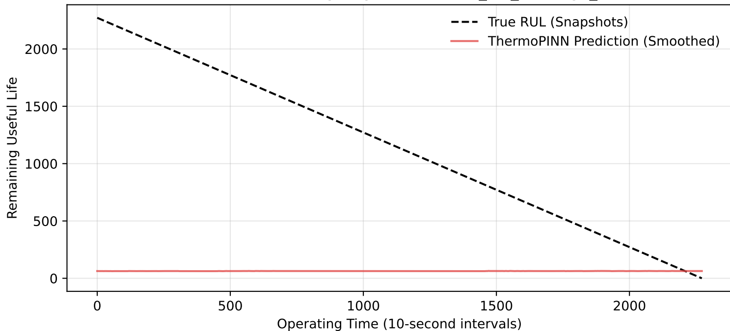
Zero-Shot Bearing Degradation: Test_set_Bearing1_5
