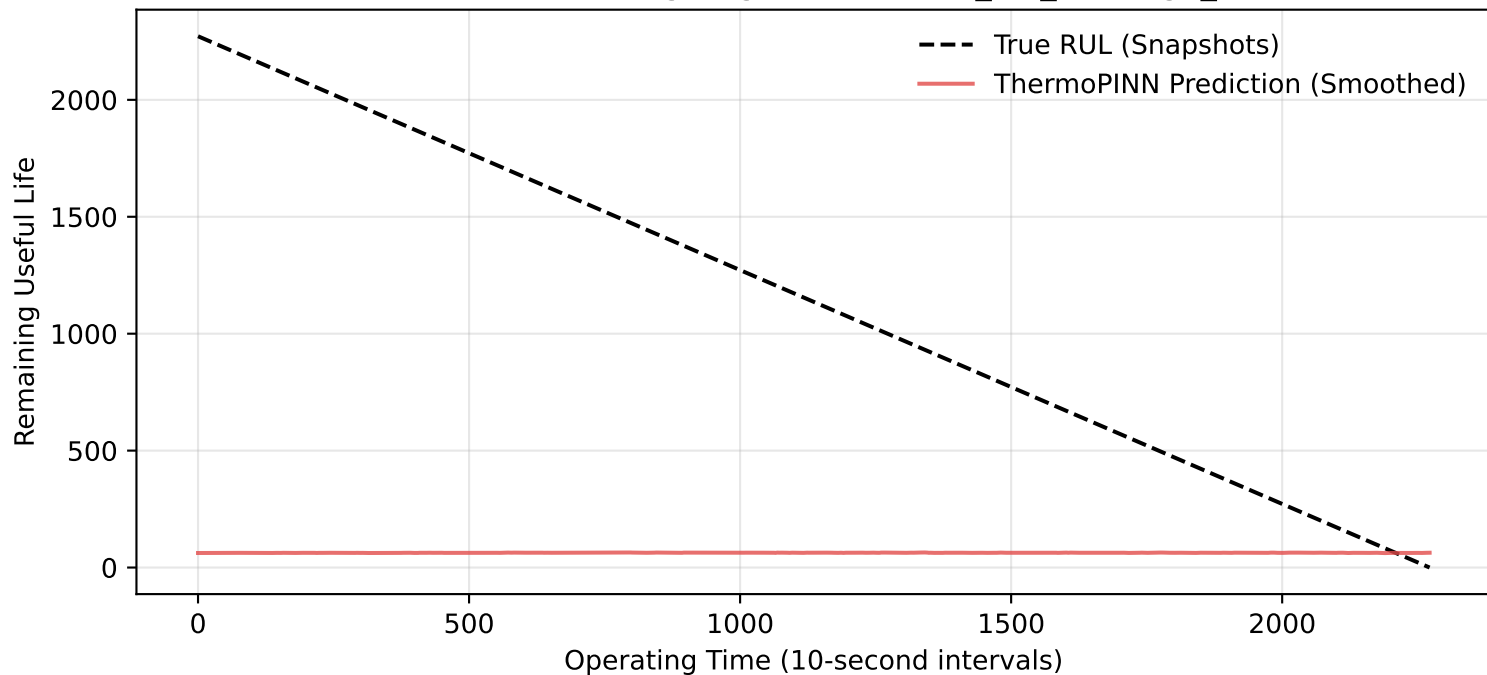
Zero-Shot Bearing Degradation: Test_set_Bearing1_6
