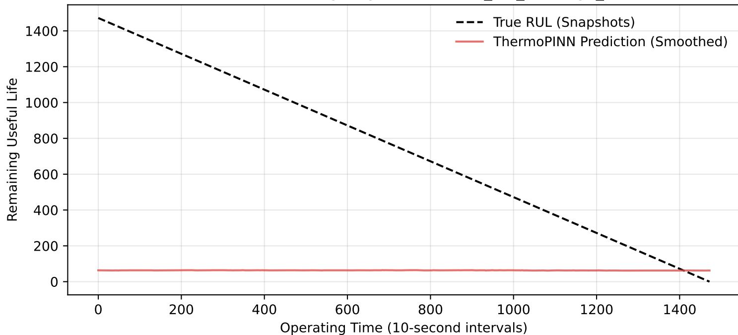
Zero-Shot Bearing Degradation: Test_set_Bearing1_7
