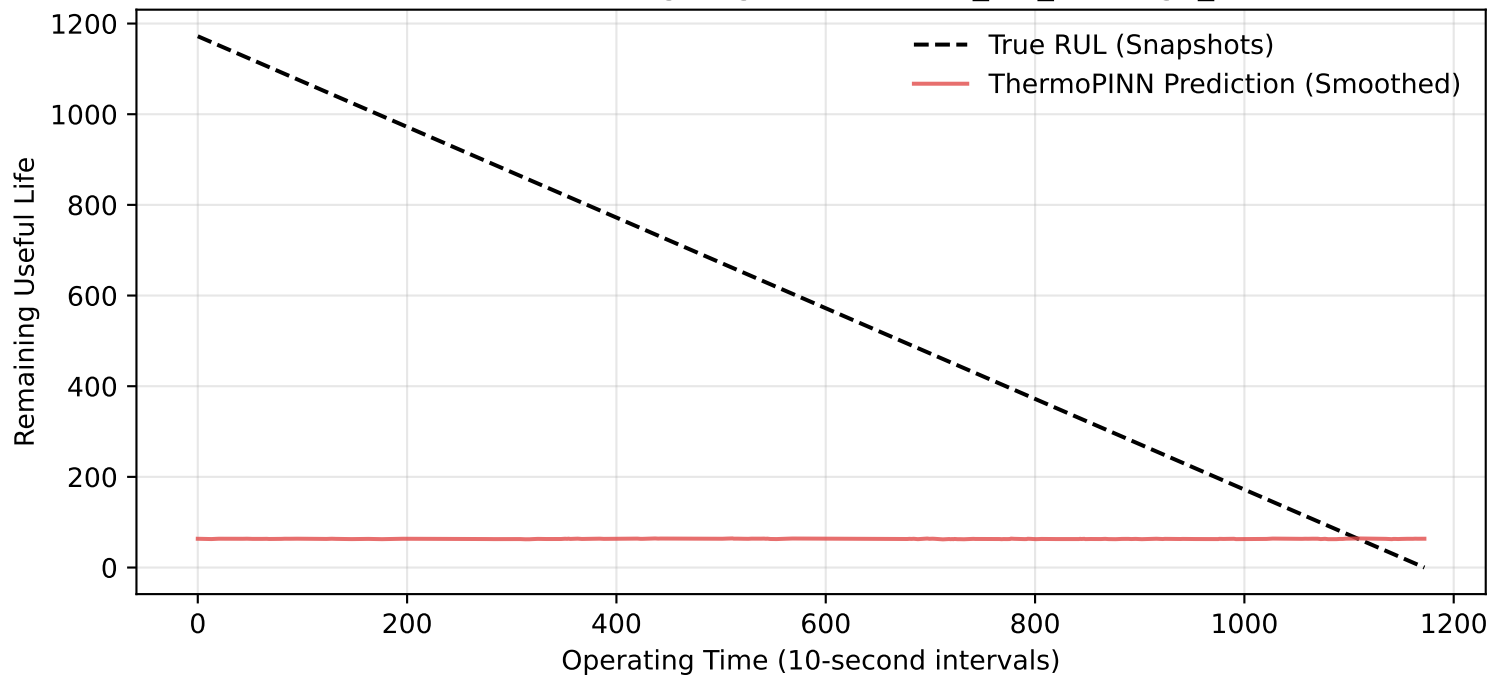
Zero-Shot Bearing Degradation: Test_set_Bearing2_3
