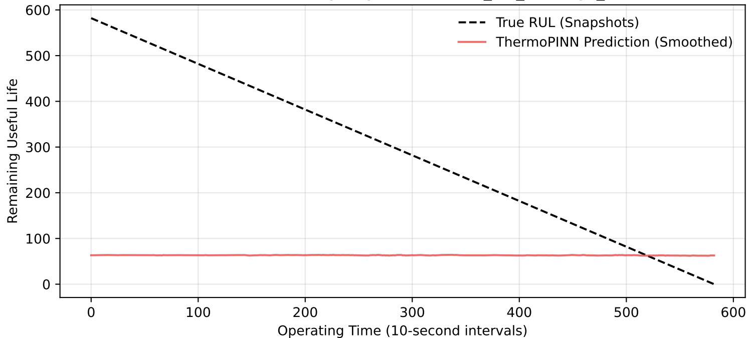
Zero-Shot Bearing Degradation: Test_set_Bearing2_4
