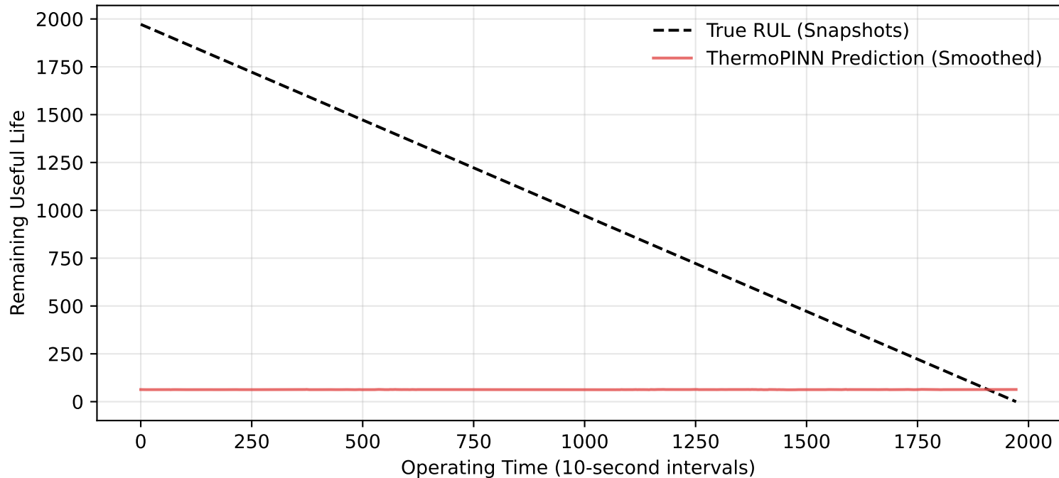
Zero-Shot Bearing Degradation: Test_set_Bearing2_5
