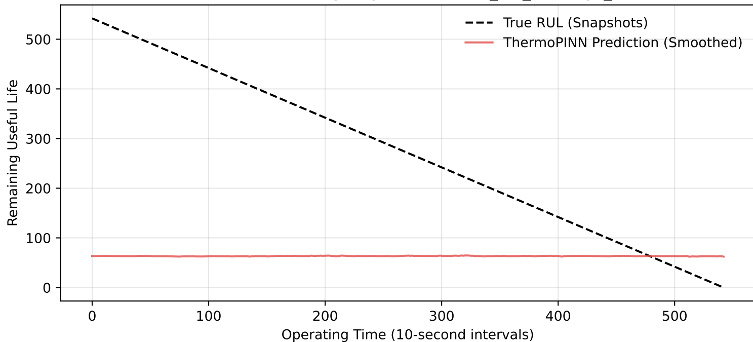
Zero-Shot Bearing Degradation: Test_set_Bearing2_6
