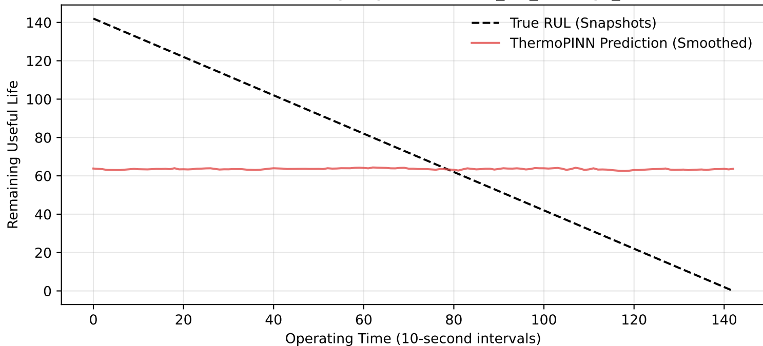
Zero-Shot Bearing Degradation: Test_set_Bearing2_7
