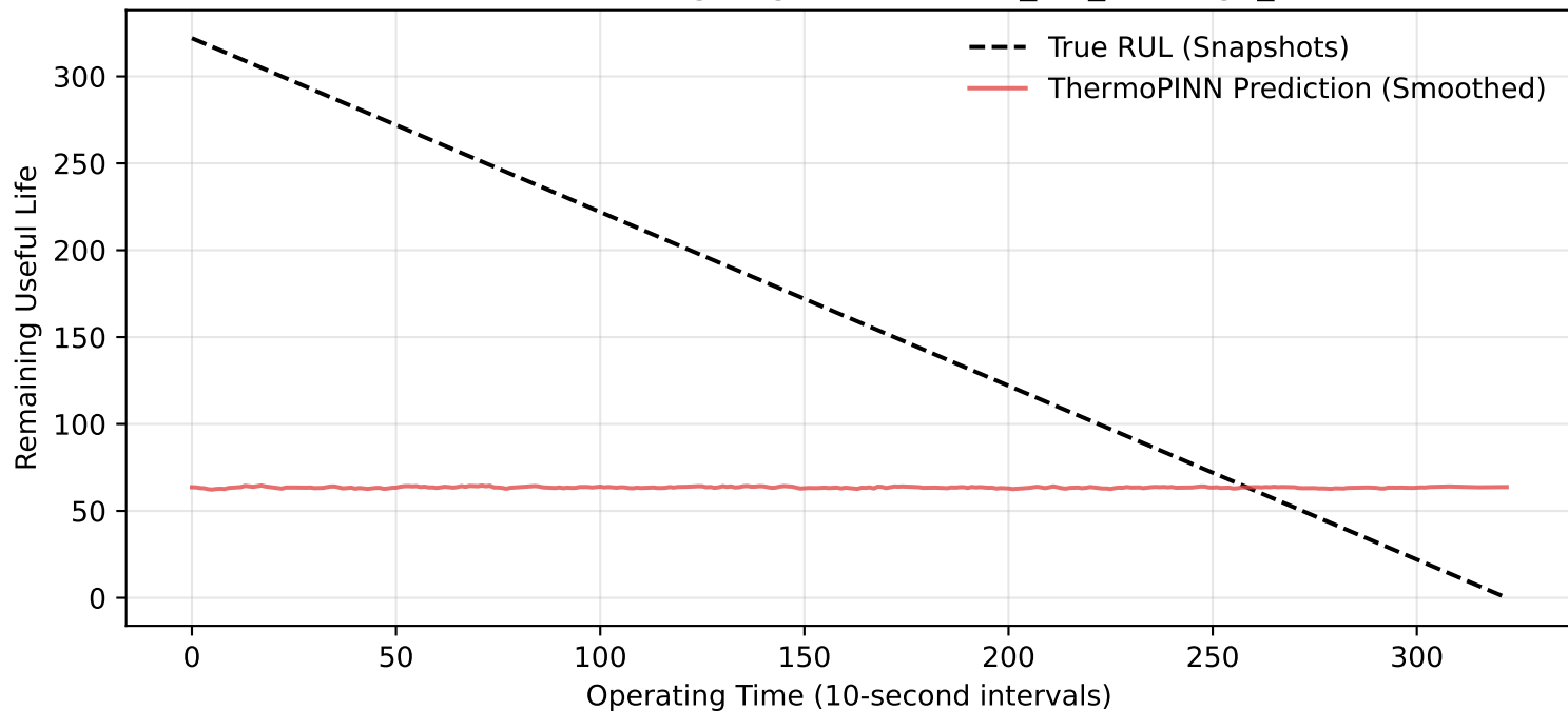
Zero-Shot Bearing Degradation: Test_set_Bearing3_3
