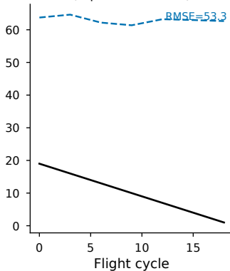
Challenging case (rapid EOL decline)
