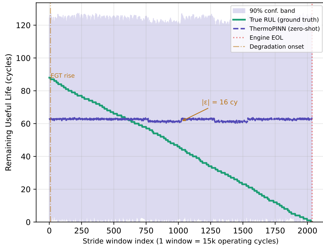
Engine 5 — N-CMAPSS_DS02-006 RMSE = 31.3 cy · zero-shot transfer
