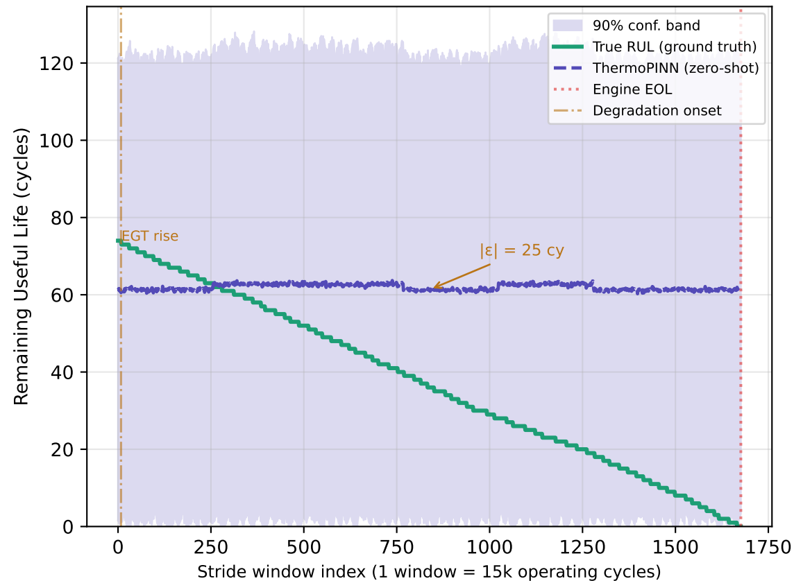
Engine 2 — N-CMAPSS_DS02-006 RMSE = 32.6 cy · zero-shot transfer
