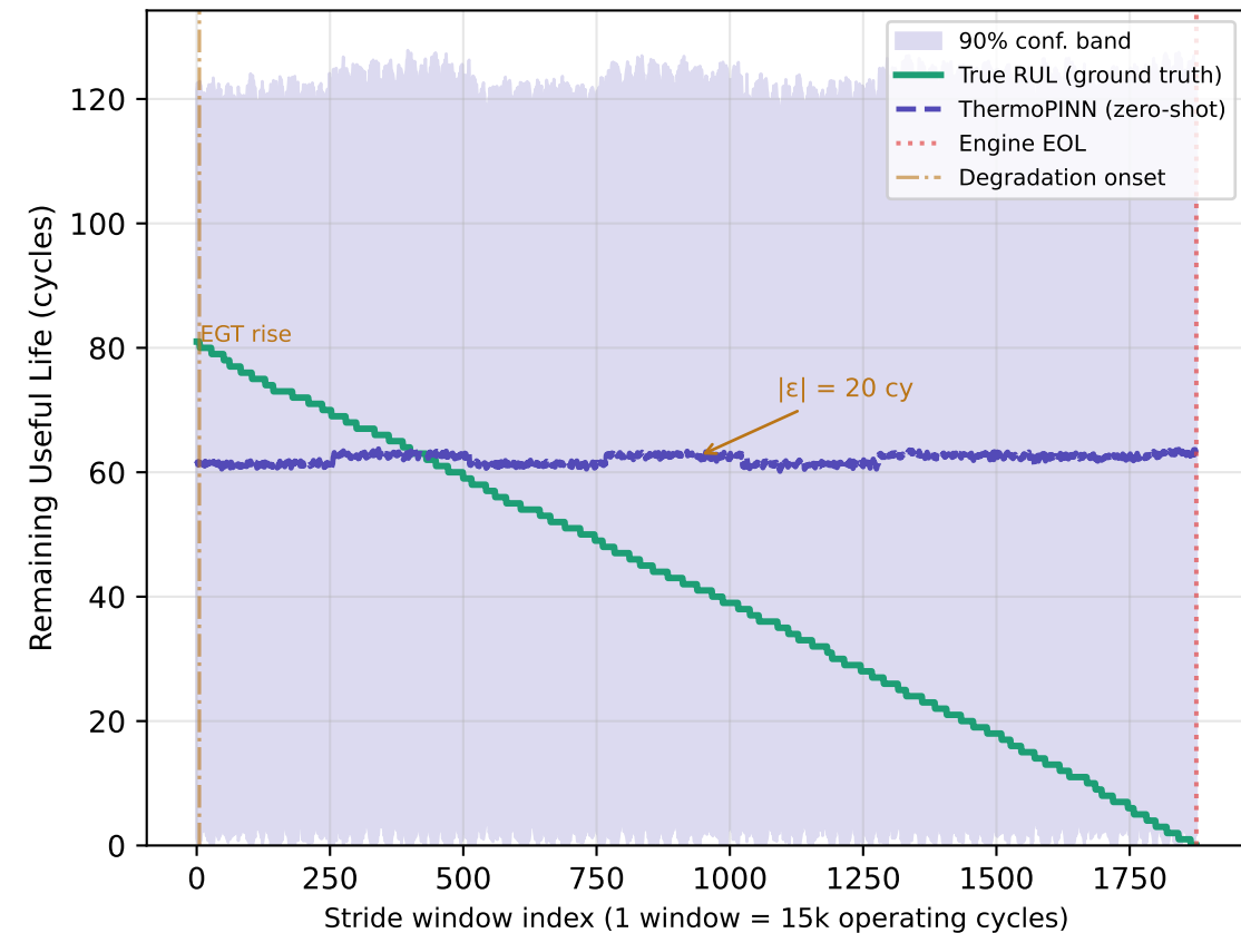
Engine 10 — N-CMAPSS_DS02-006 RMSE = 31.3 cy · zero-shot transfer
