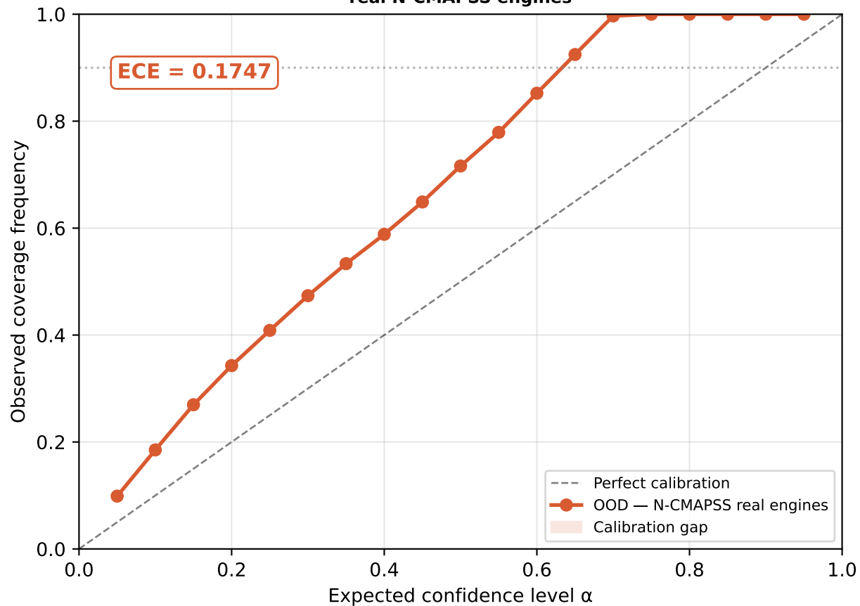
(b) OOD calibration (ECE=0.1747) real N-CMAPSS engines
