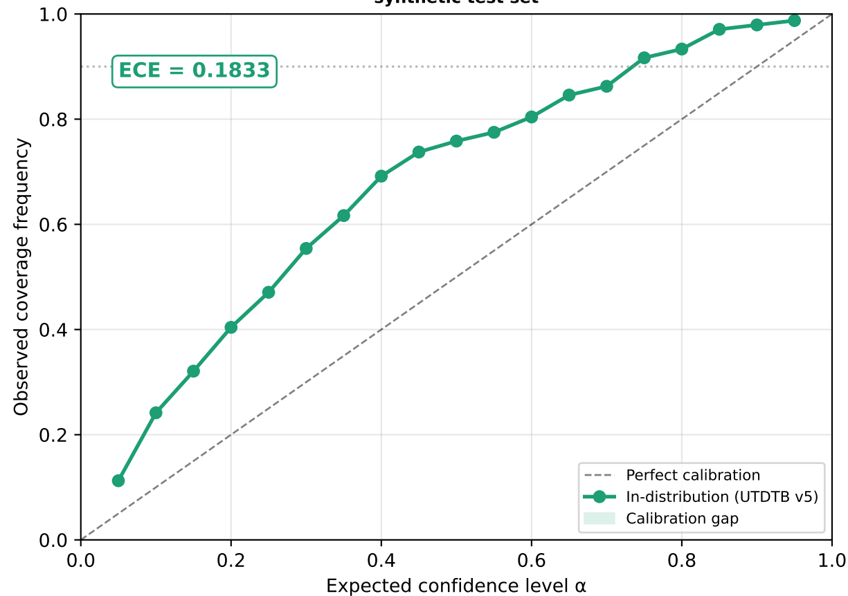
(a) ID calibration (ECE=0.1833) synthetic test set
