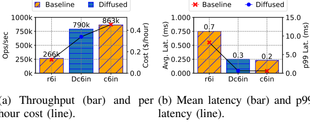
Fig. 8: Memcached with r6i.large (2 vCPU, 16 GiB memory) and c6in.2xlarge (8 vCPU, 16 GiB memory) instances, loaded with 20 M 640 bytes records totalling 14 GiB. Baseline: running without DIFFUSED on r6i and c6in instances. DIFFUSED: roaming from r6i instance to the c6in instance.
