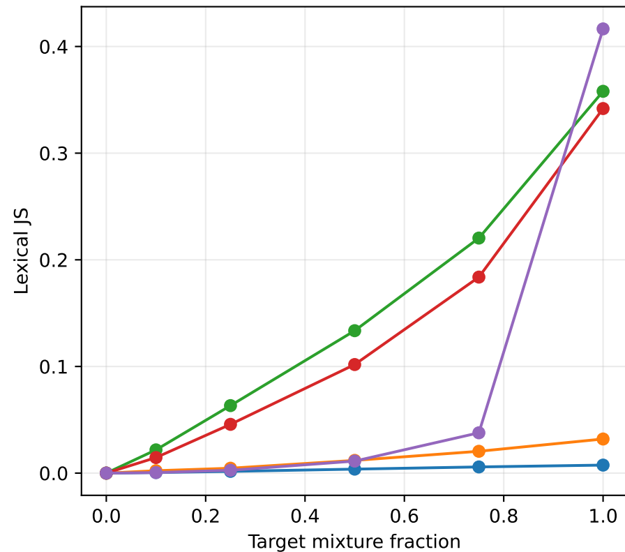
Mixture lexical movement
