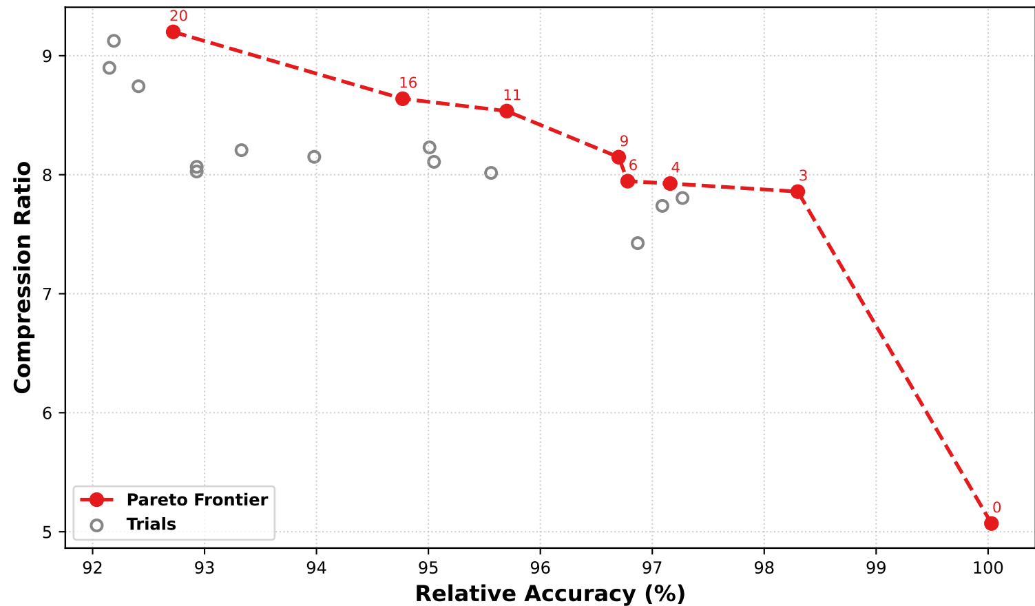
Meta-Llama-3.1-8B-Instruct none transform Pareto Frontier
