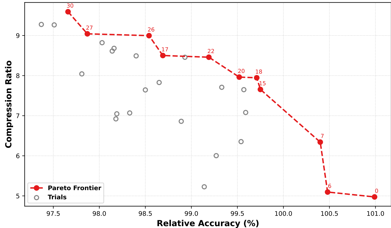
Qwen2.5-7B-Instruct Pareto Frontier
