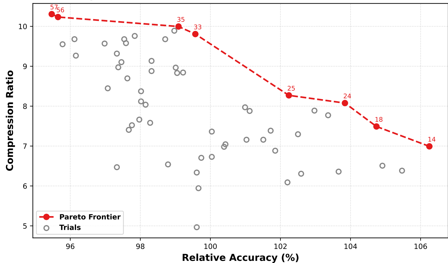
Qwen2.5-7B-Instruct hadamard transform Pareto Frontier
