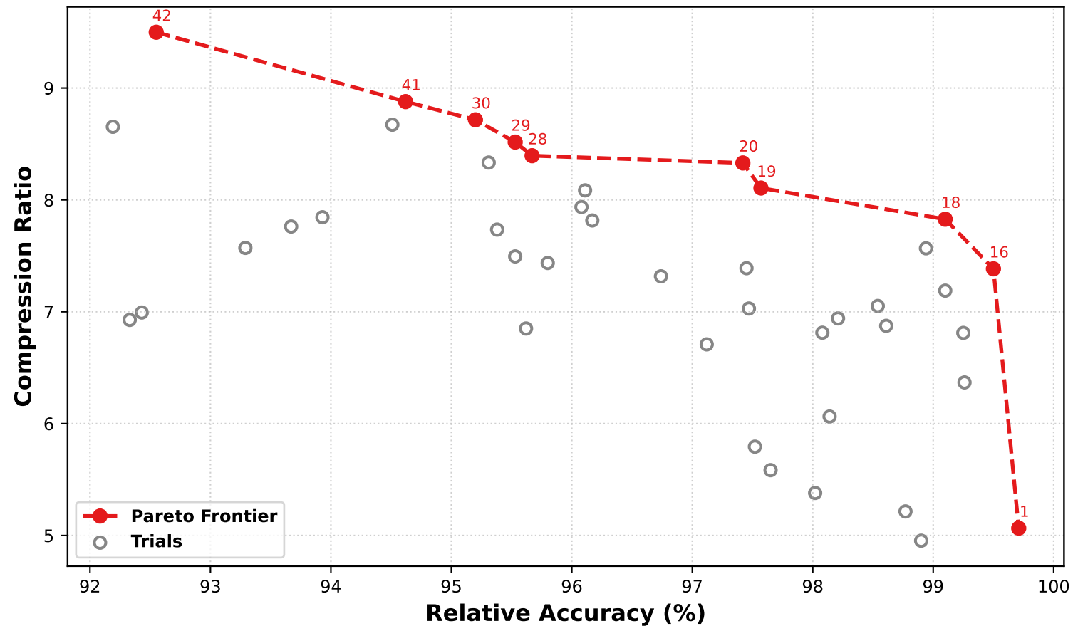
Qwen2.5-7B-Instruct none transform Pareto Frontier
