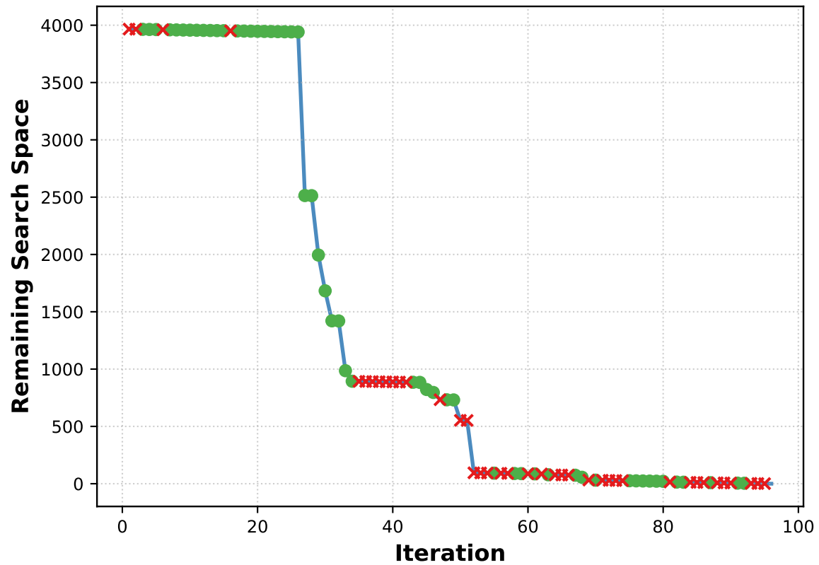
Pruning Process
