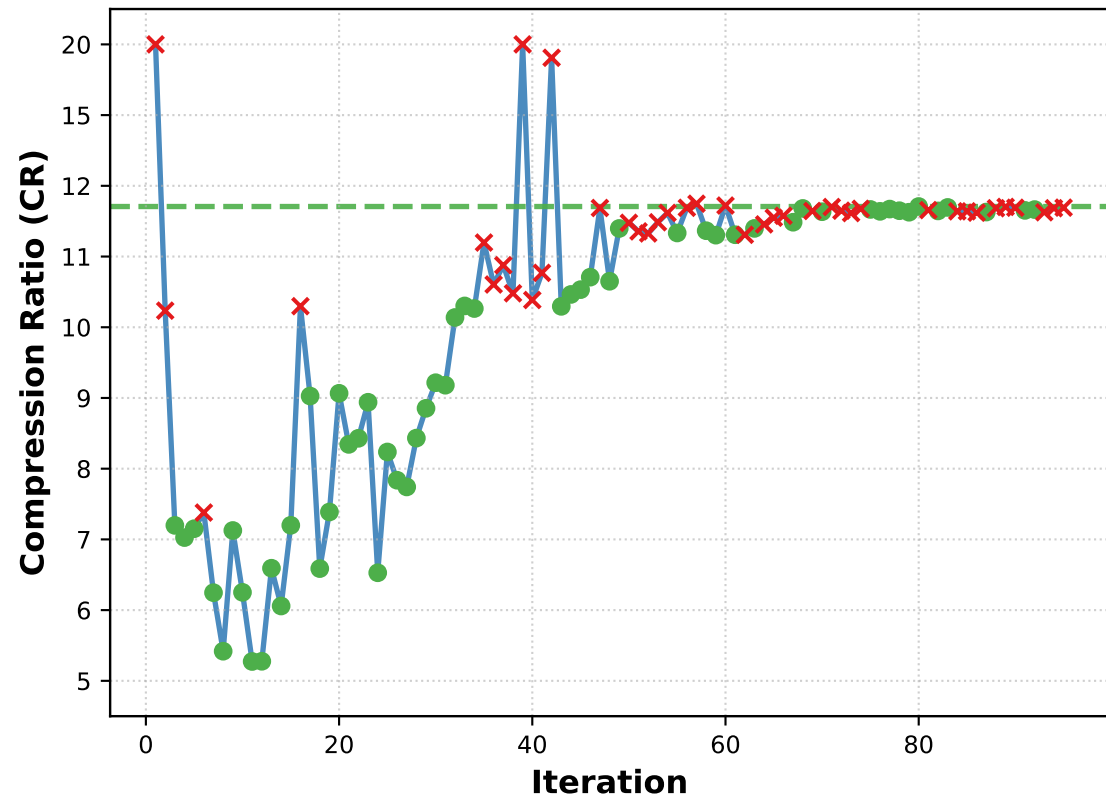
Exploration Process
