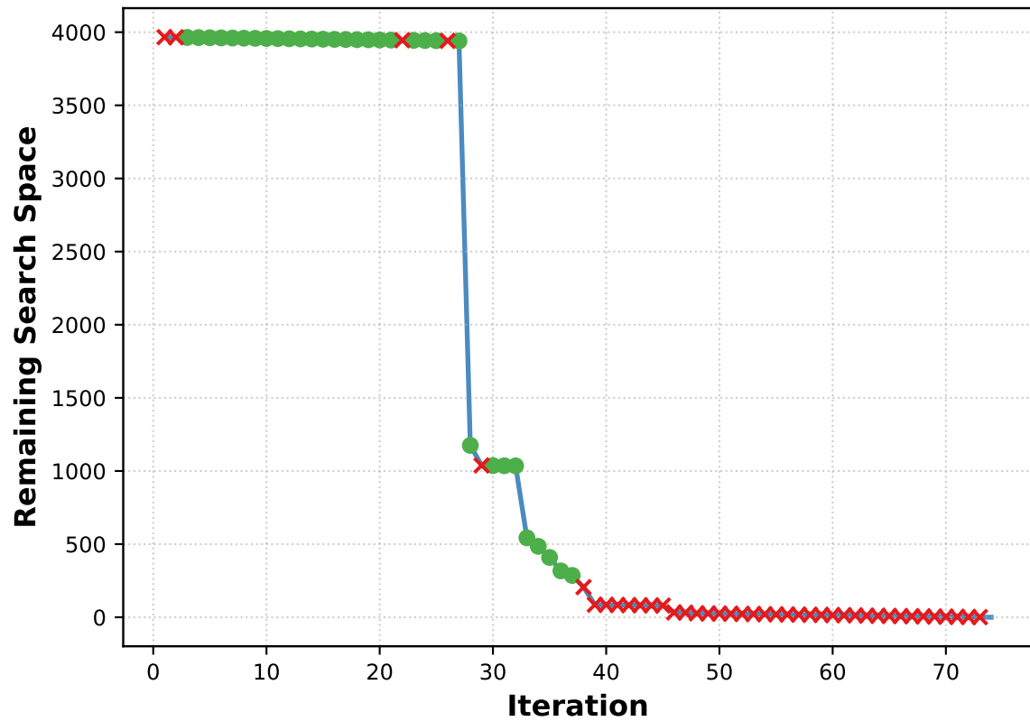
Pruning Process
