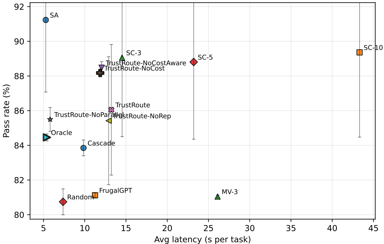
GSM8K: Pass rate vs Avg latency (s per task)
