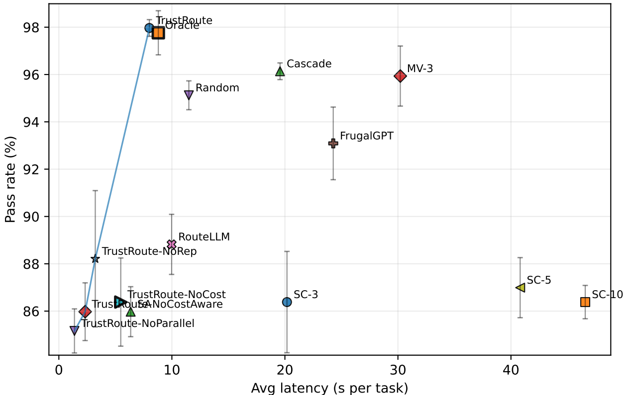
HumanEval: Pass rate vs Avg latency (s per task)
