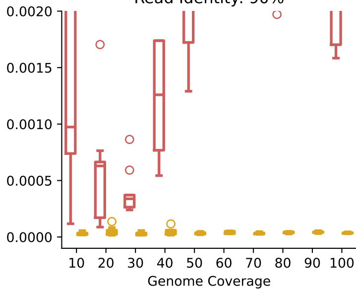
Read Identity: 90%
