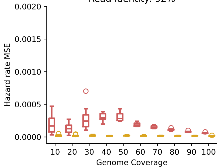
Read Identity: 92%
