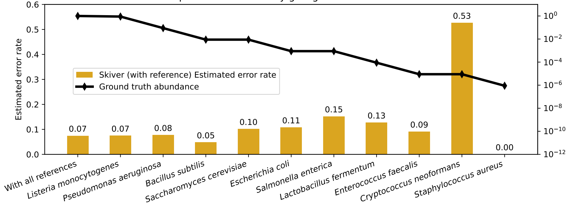
Estimated per-base error rate by giving skiver individual references
