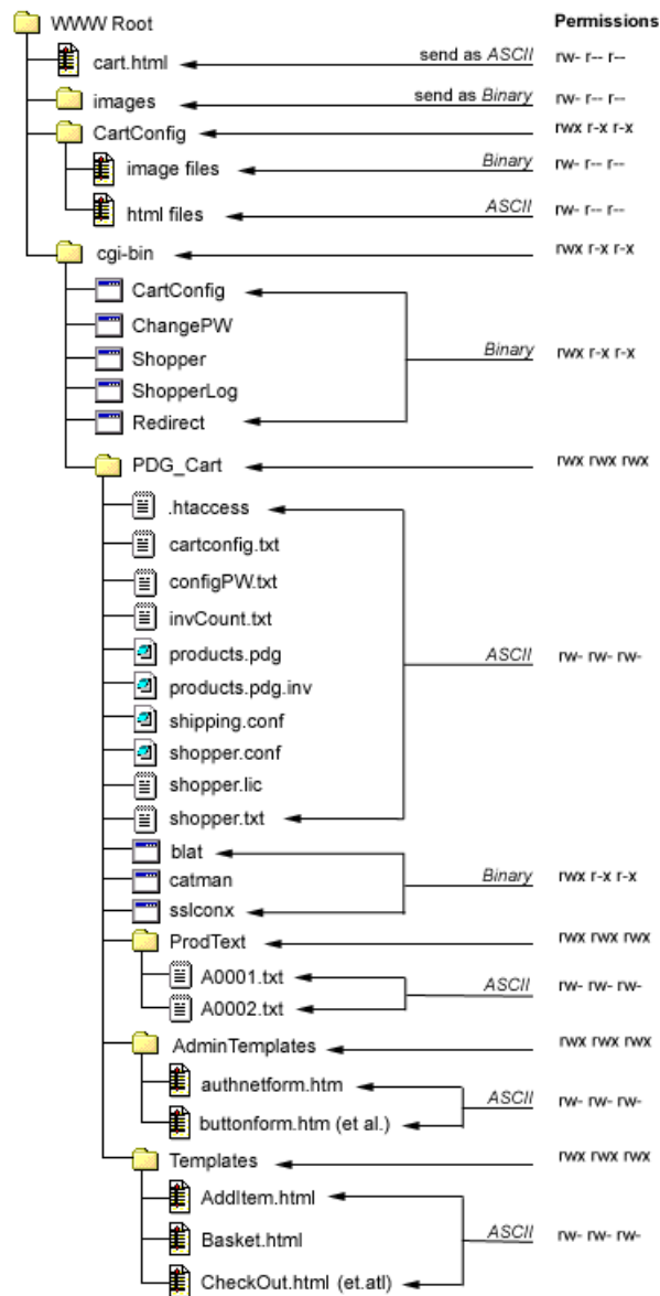
Figure 4-1 Complete PDG Shopping Cart File Structure
